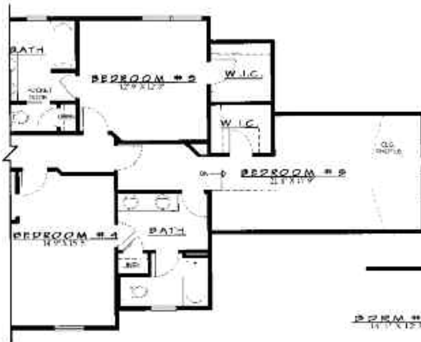
SECOND FLOOR PLAN W/ 5TH BEDROOM OPT. (BASED ON ELEV. 'N')
