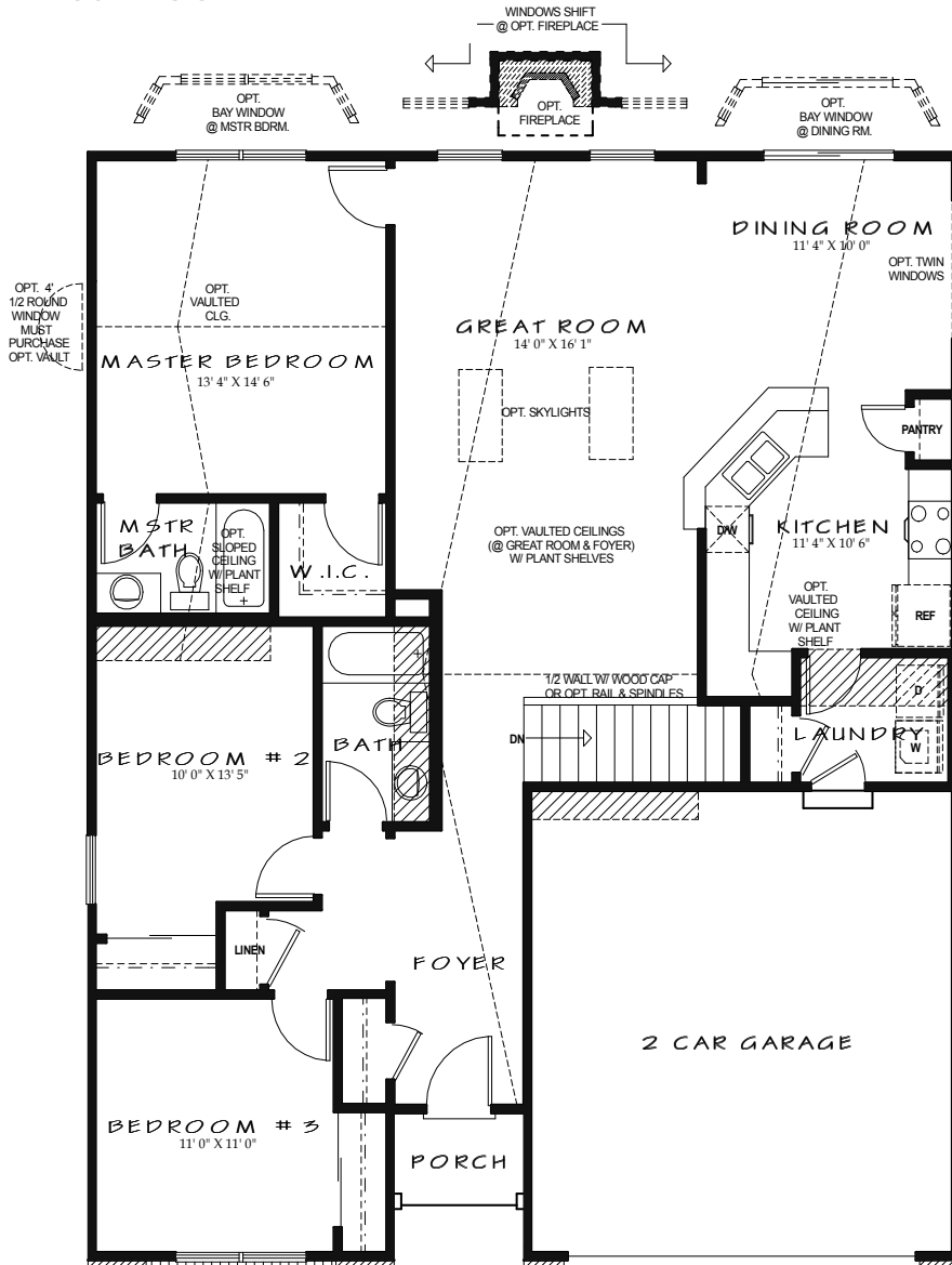
FIRST FLOOR PLAN (BASED ON ELEV. "A")
