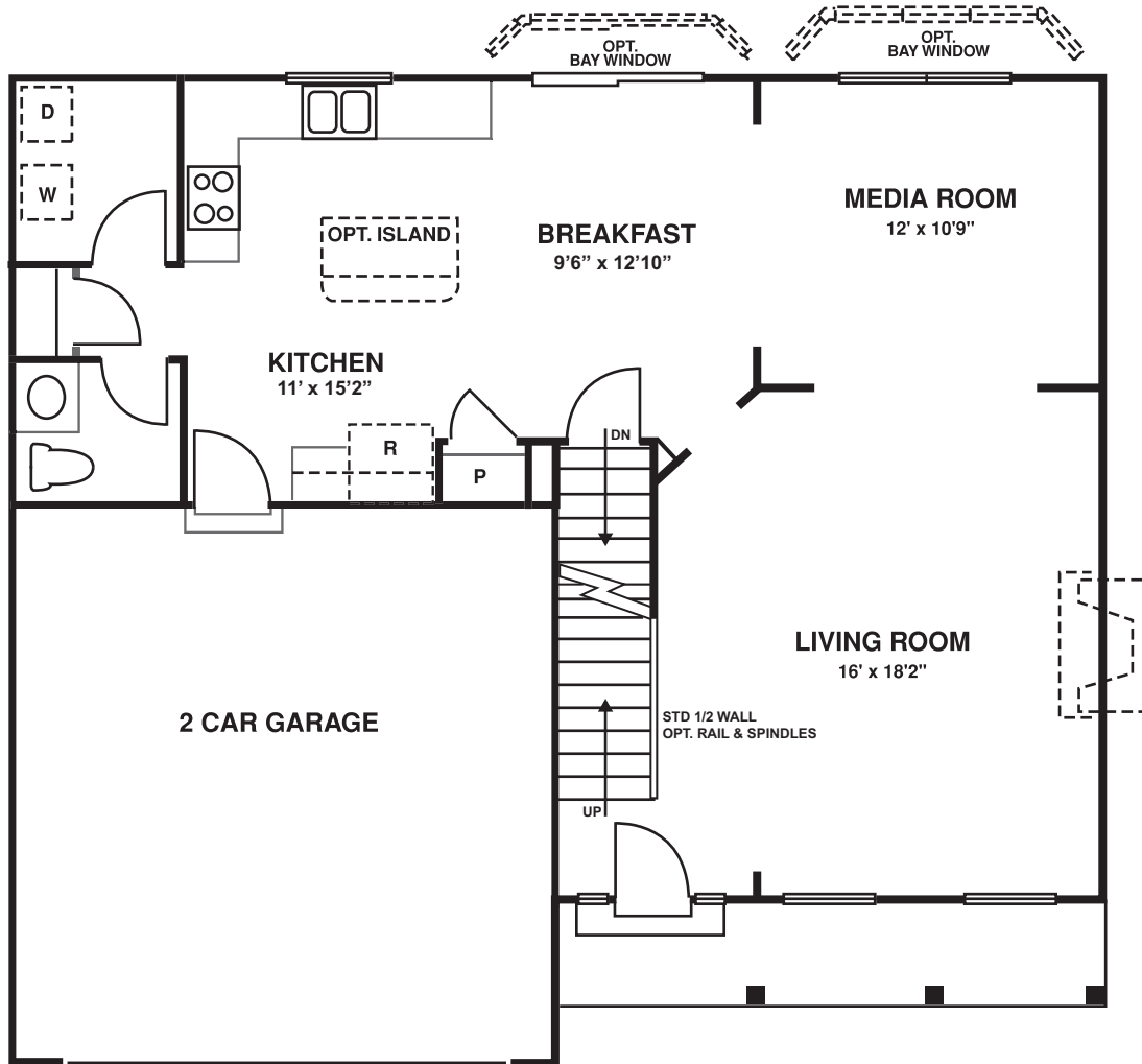
FIRST FLOOR PLAN BASED ON ELEVATION A
