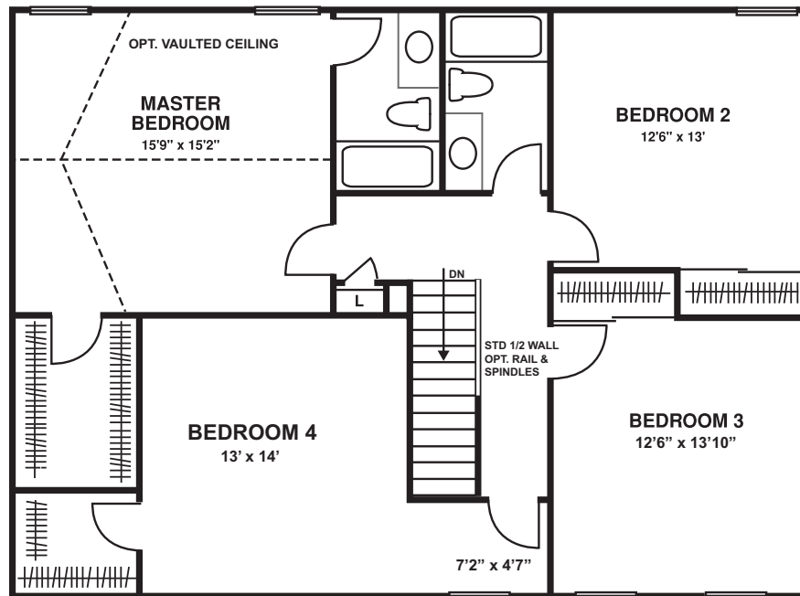
OPT. 4 BEDROOM PLAN
