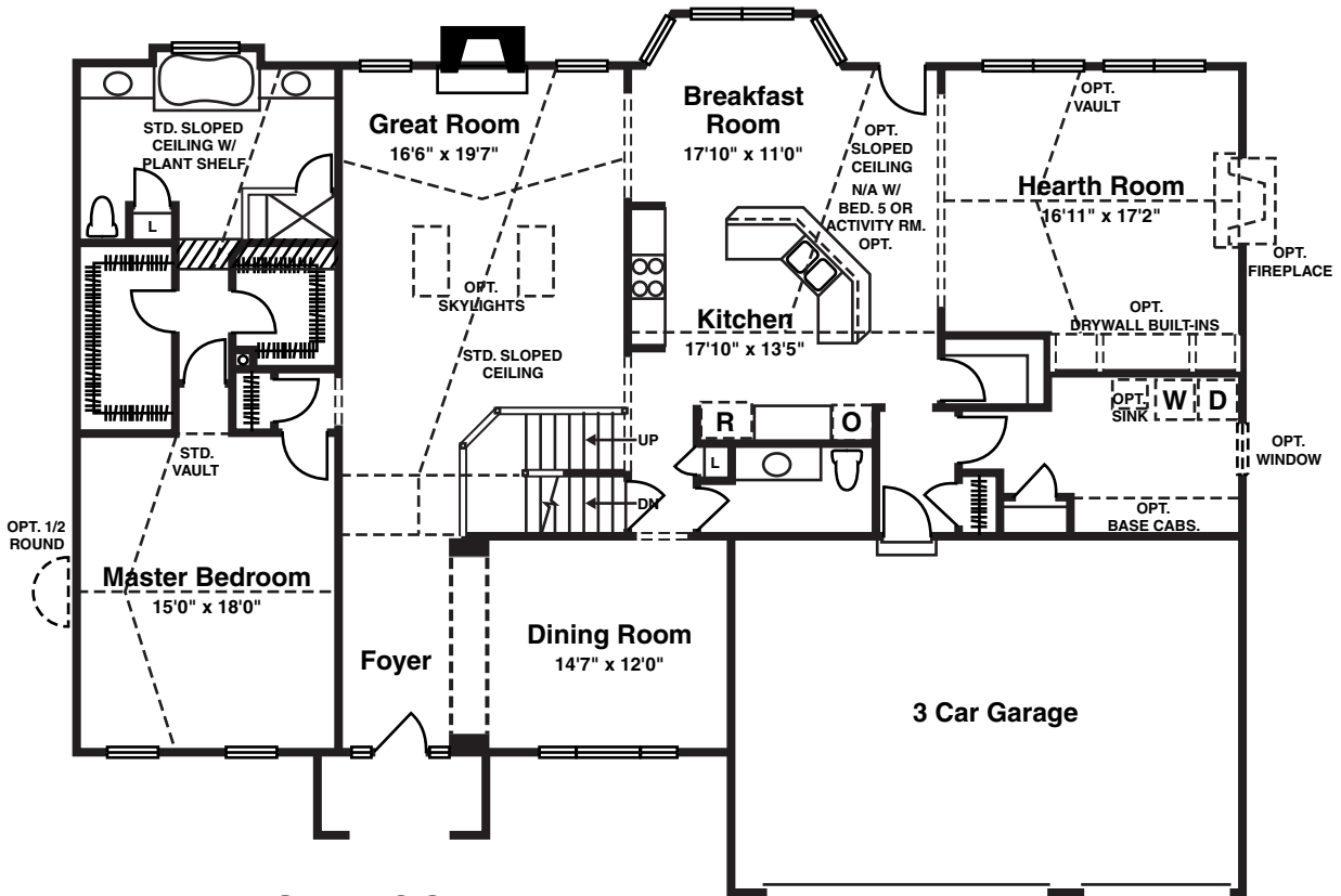
FIRST FLOOR PLAN (BASED ON ELEVATION A)
