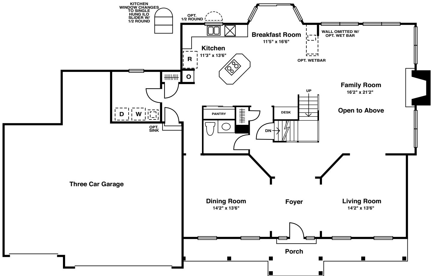
FIRST FLOOR PLAN (Based on Elevation B)
