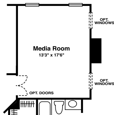
OPTIONAL MEDIA ROOM ILO 2 STORY GREAT ROOM
