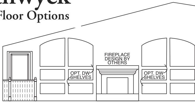
ELEVATION AT GREAT ROOM
