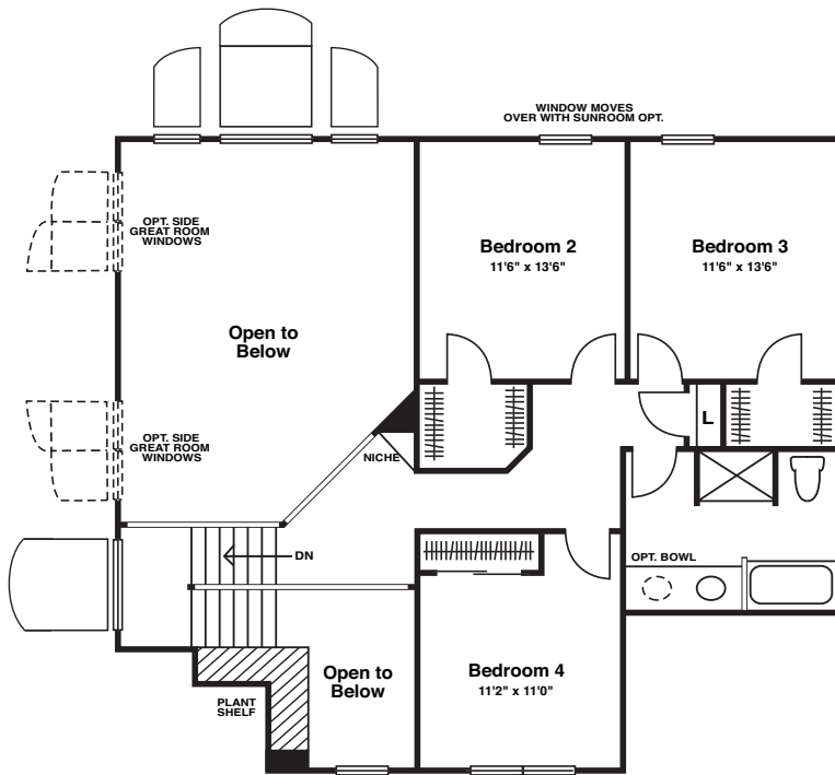
SECOND FLOOR PLAN (BASED ON ELEV. "B")
