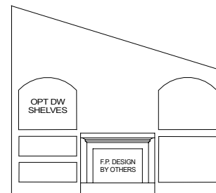
OPT. DRYWALL SHELVES @ EACH SIDE OF FIREPLACE
