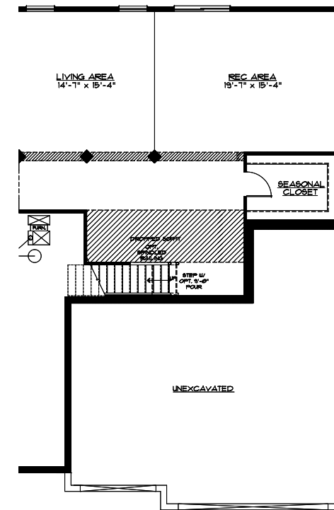
OPT. FINISHED LOWER LEVEL PLAN W/ OPT. MODULE "B"
