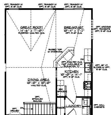
OPT. INVERTED VAULTED CEILING
