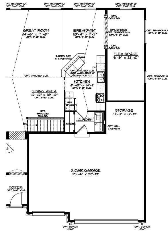
1ST FLOOR PLAN W/ OPT. MODULE "B"
