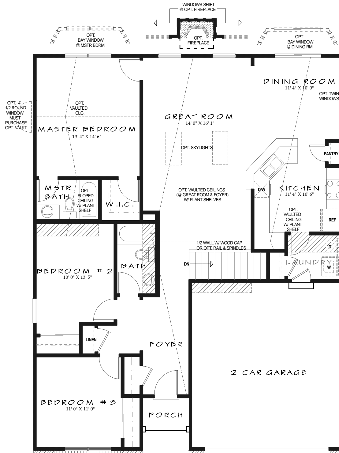
FIRST FLOOR PLAN (BASED ON ELEV. 'A')
